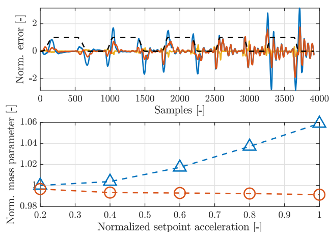
Figure 2: Top: error signals of linear (—), the developed (—), and NOILC (—) approach. Bottom: mass per setpoint acceleration of linear (—△) and the developed (—○) approach.
