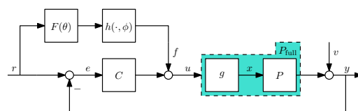
Figure 1: Proposed control scheme with Wiener feedforward f = h(F(\theta)r, \phi) .
