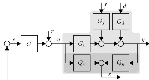
Figure 1: Closed-loop configuration for fault detection by means of the residual signal \varepsilon . The residual generator, Q(s) (■), and the open-loop problem (□) are indicated.
