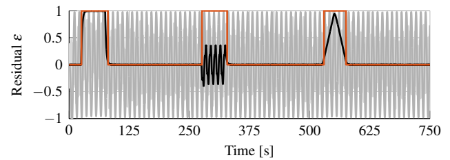
Figure 2: Comparison between normalized effective residual (—) with fault flag (—), and residual signals based on classical design techniques (—), (—).
